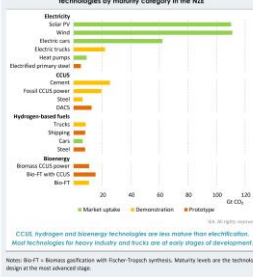
Figure 2.32 – Cumulative CO 2 emissions reductions for selected technologies by maturity category in the NZE
