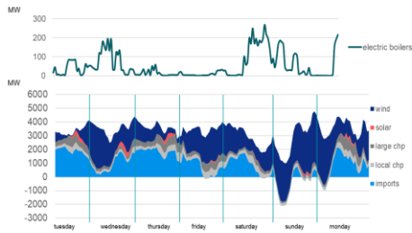
FLEXIBILITY FROM THE ENERGY MIX A RANDOM WEEK – NOVEMBER 17-23, 2020
