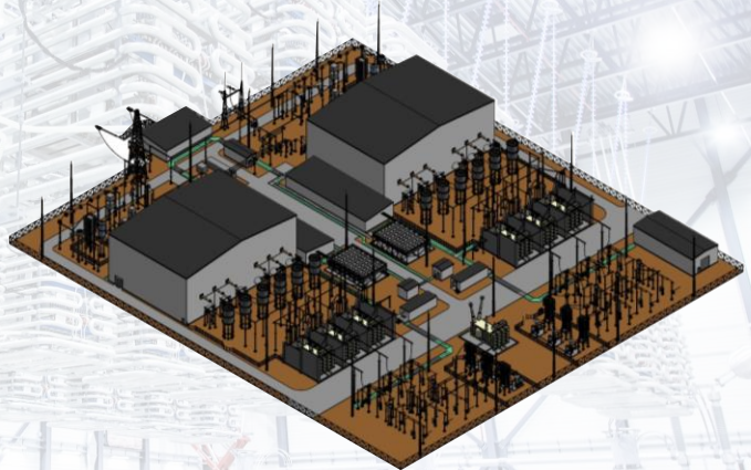
双極 ( \pm 525 \text{ kV} ) 2,000 – 3,000 MW
