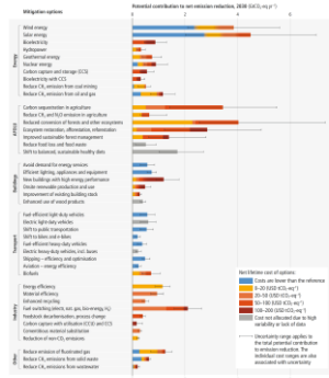
Figure 2M2 | Overview of mitigation options and their estimated ranges of costs and potentials in 2050
